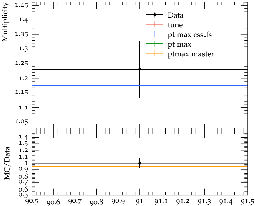
Mean \rho^0(770) multiplicity
