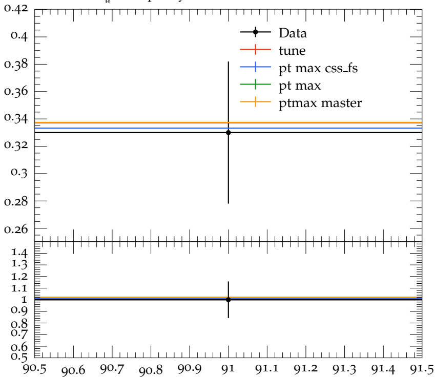
Mean B^+, B_d^0 multiplicity
