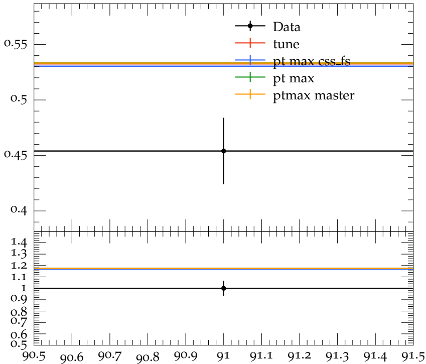
Mean D^0 multiplicity
