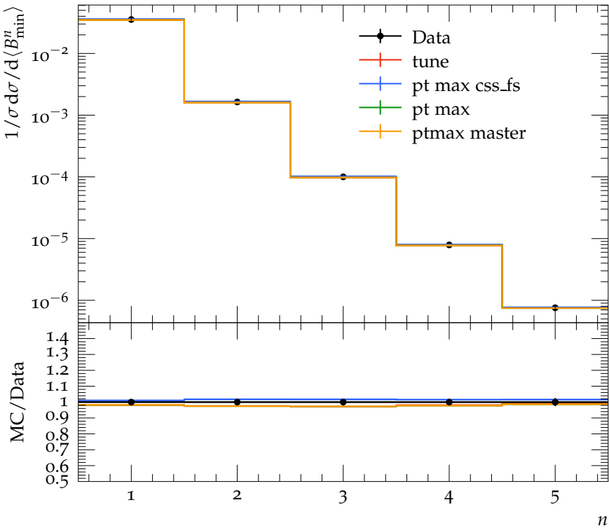
Moments of B_{\min} at 91 GeV
