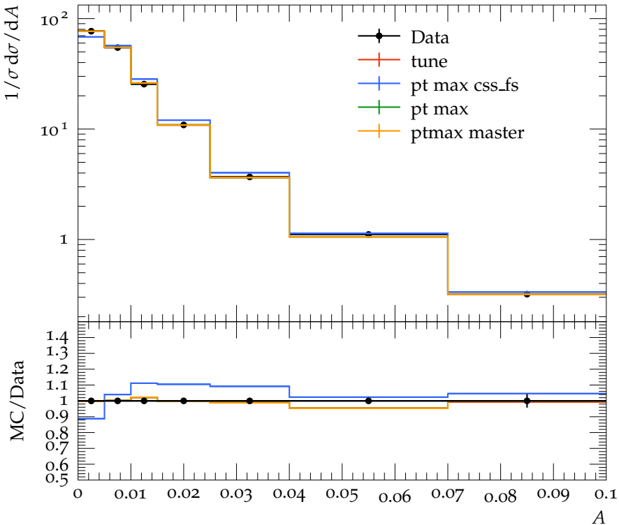
Aplanarity, A , at 91 GeV
