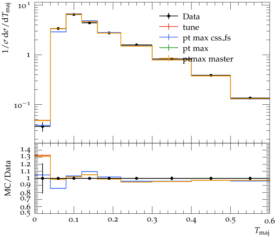
Thrust major, T_{\text{maj}} , at 91 GeV
