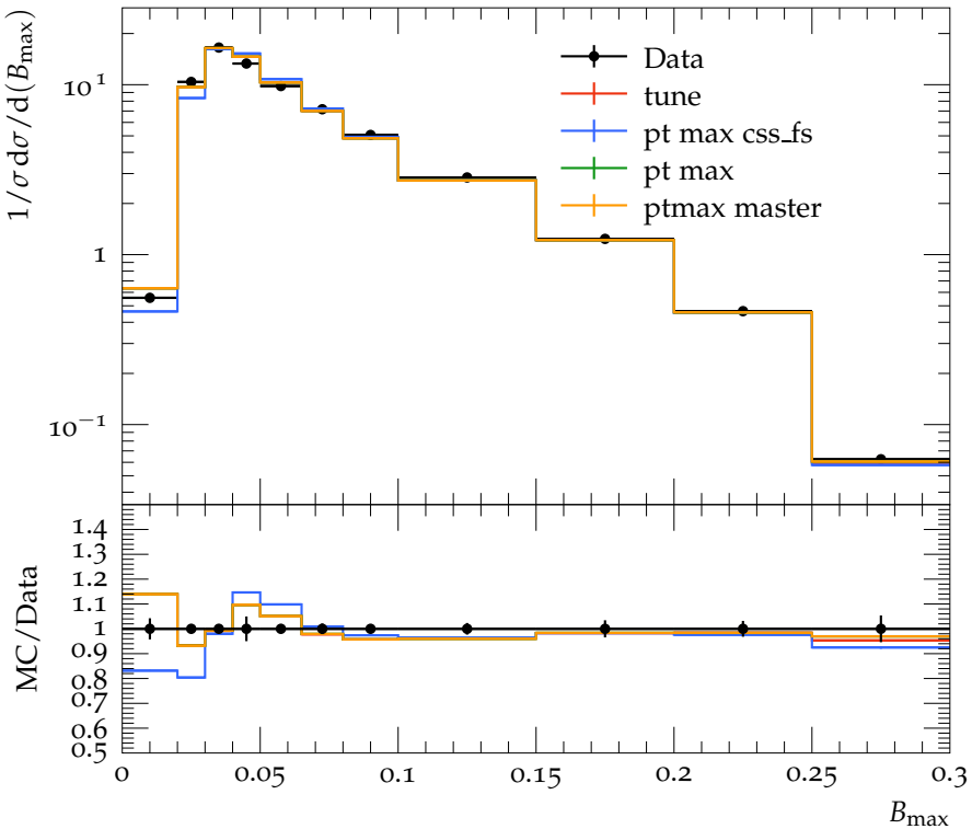
Wide hemisphere broadening, B_{\text{max}} , at 91 GeV
