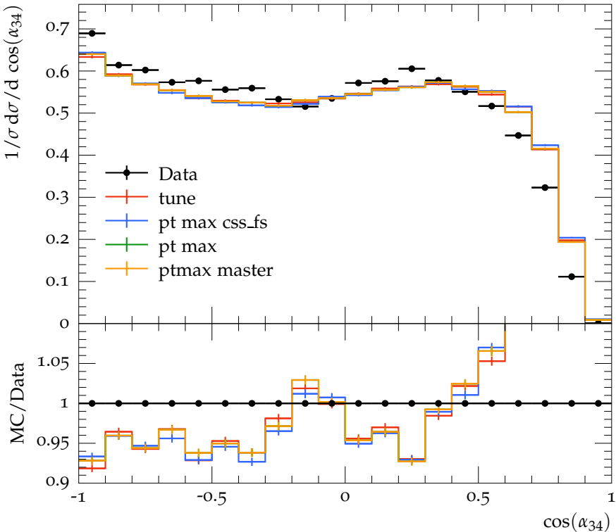
Angle between the two softest jets (parton level)
