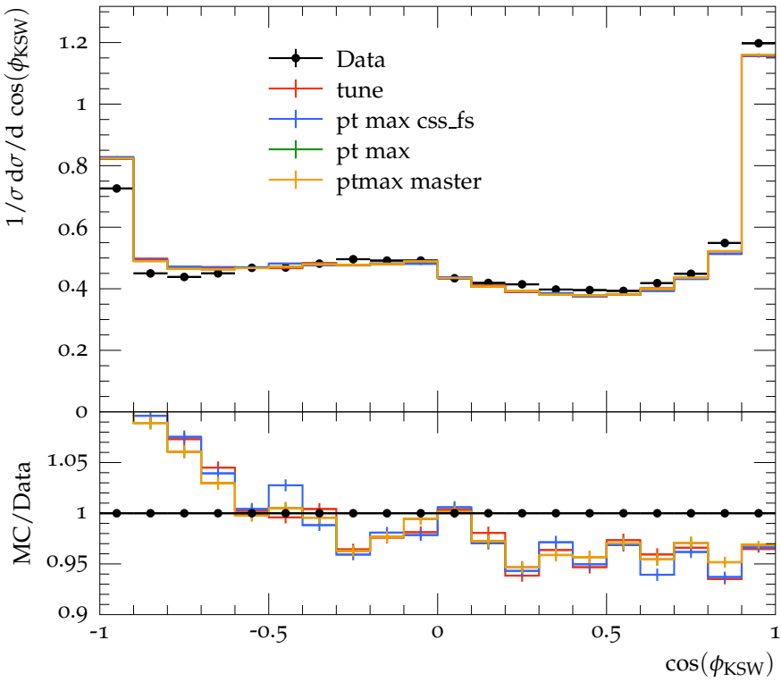
Körner-Schierholz-Willrodt angle (parton level)
