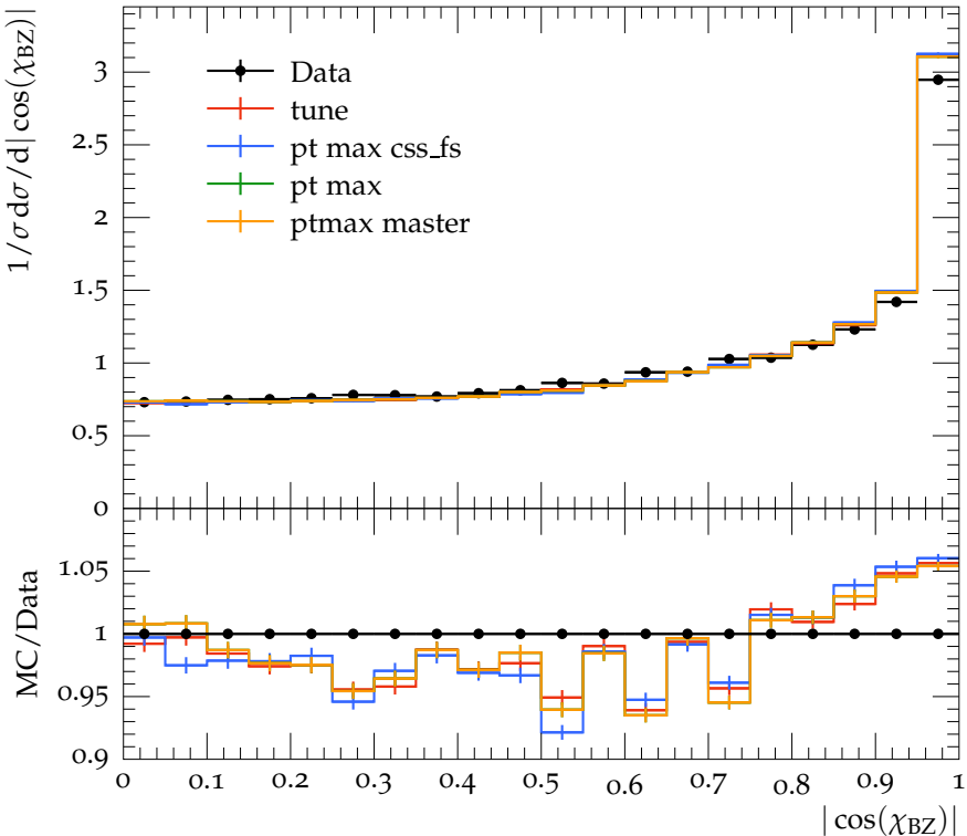
Bengtsson-Zerwas angle (parton level)
