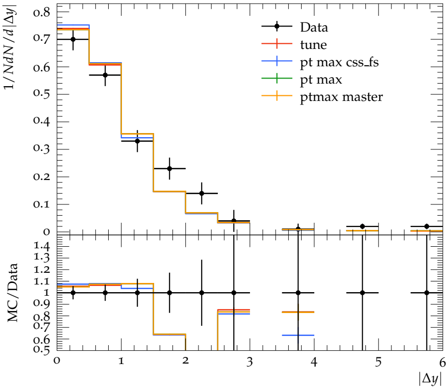
\Lambda\bar{\Lambda} correlation (2 jet events)
