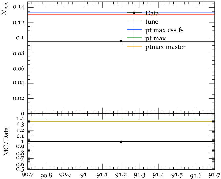
\Lambda\bar{\Lambda} pair multiplicity (3 jet events)
