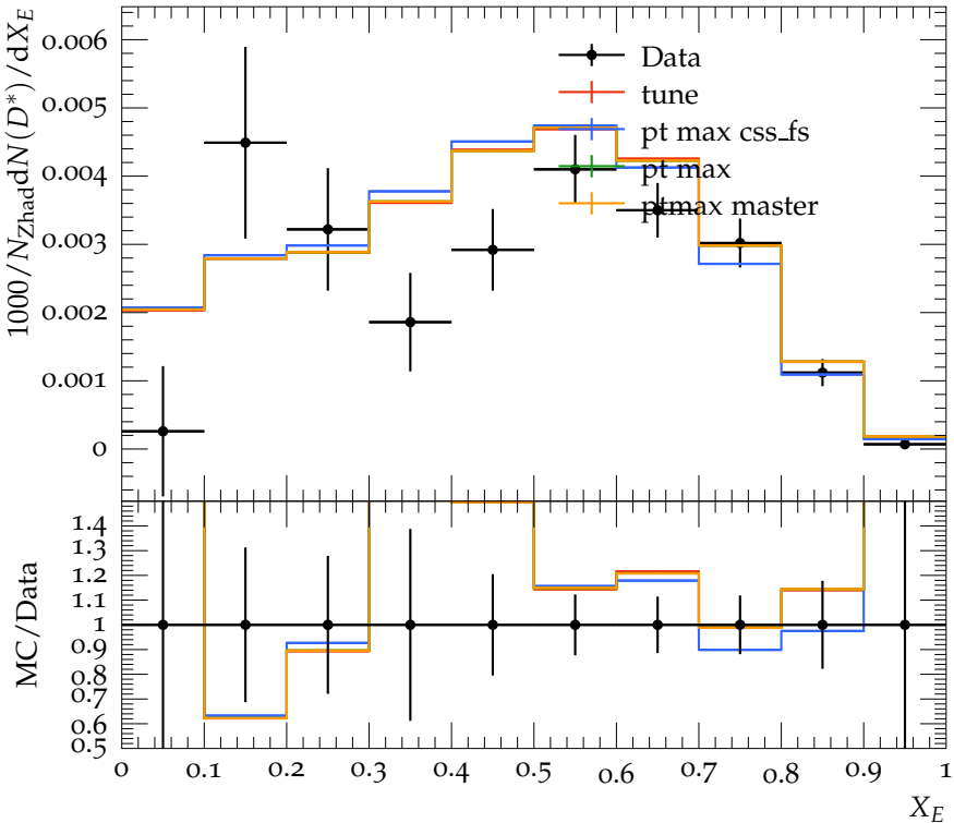
Scaled energy of D^{*\pm} in charm events at \sqrt{s} = 91.2 GeV
