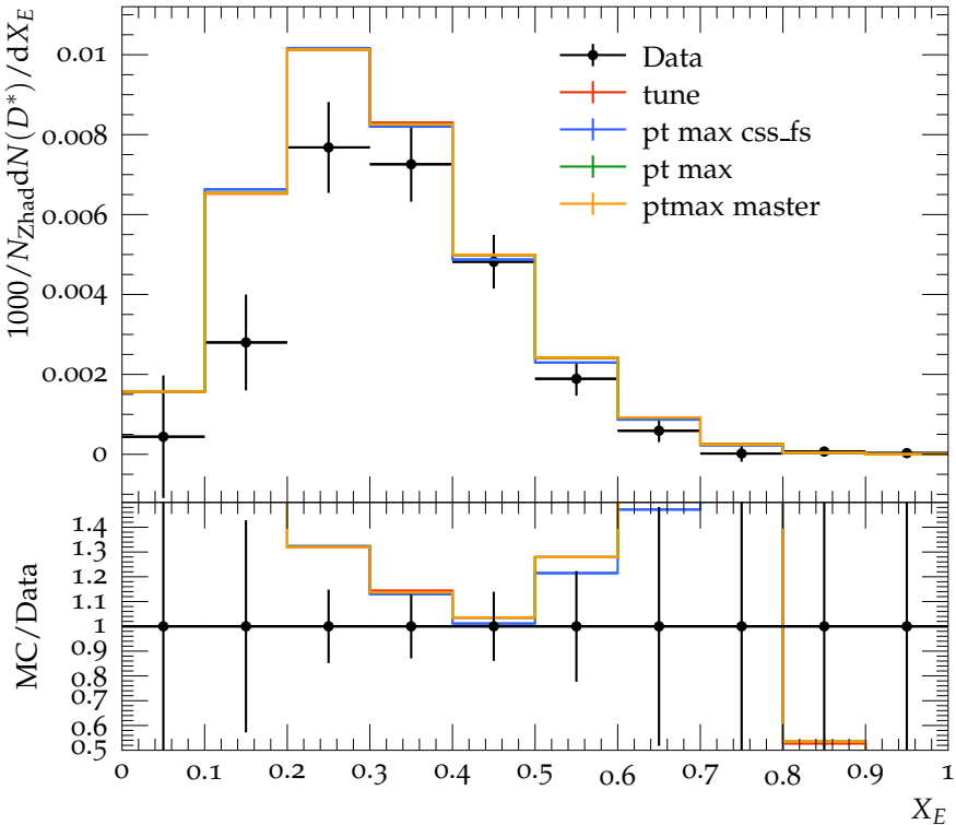
Scaled energy of D^{*\pm} in bottom events at \sqrt{s} = 91.2 GeV
