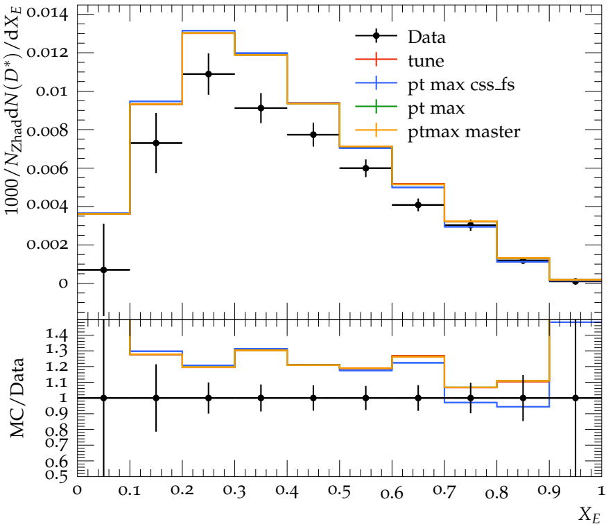
Scaled energy of D^{*\pm} at \sqrt{s} = 91.2 GeV
