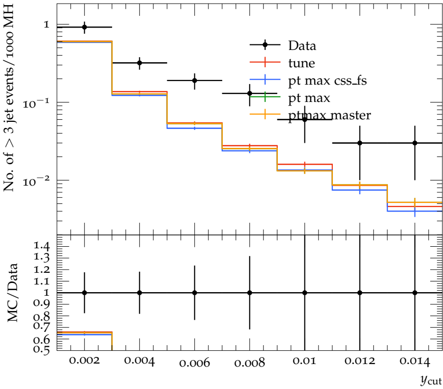
Number of > 3 jet events vs y_{\text{cut}} , Durham
