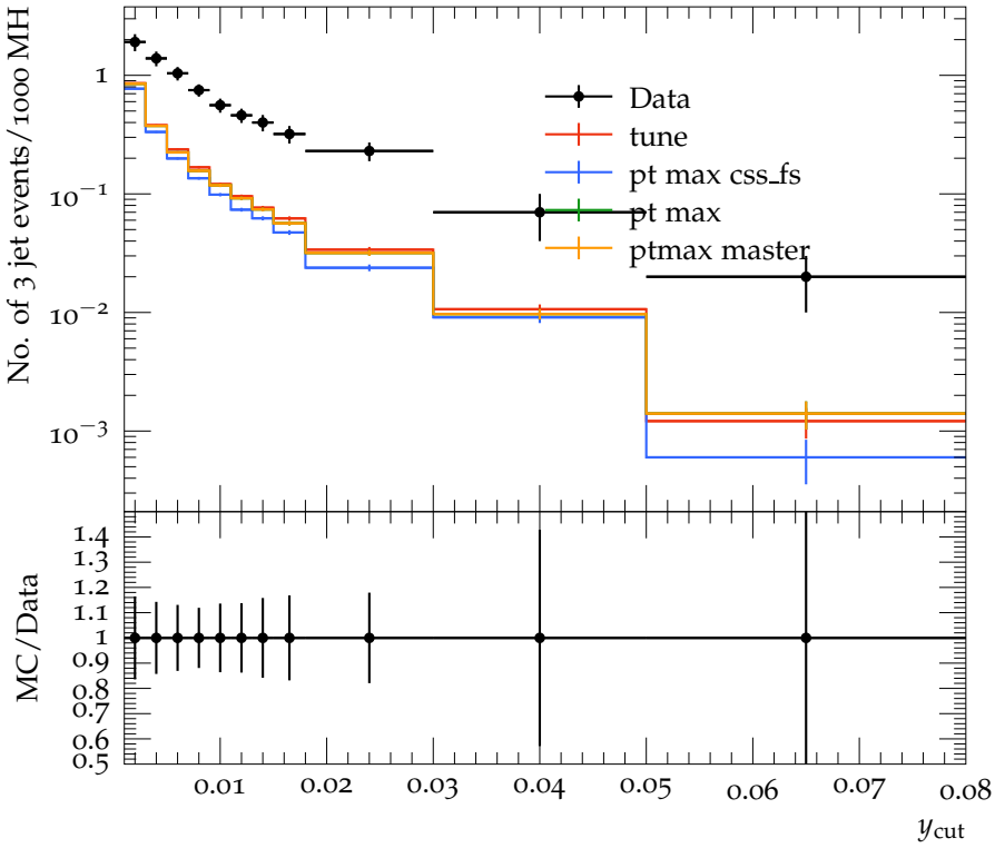
Number of 3 jet events vs y_{\text{cut}} , Durham
