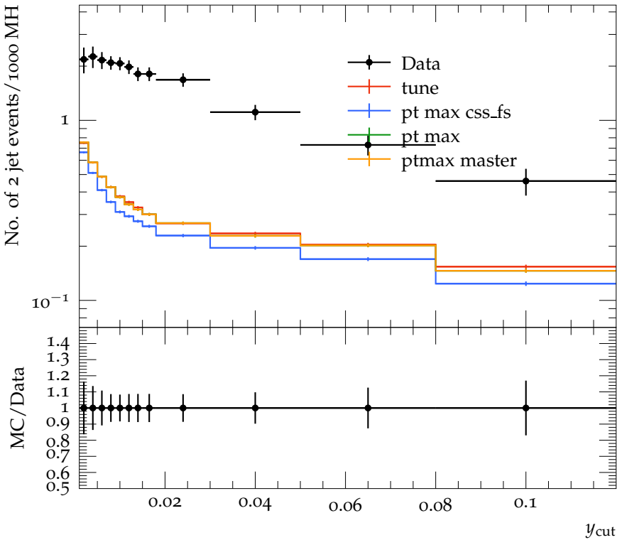
Number of 2 jet events vs y_{\text{cut}} , Durham
