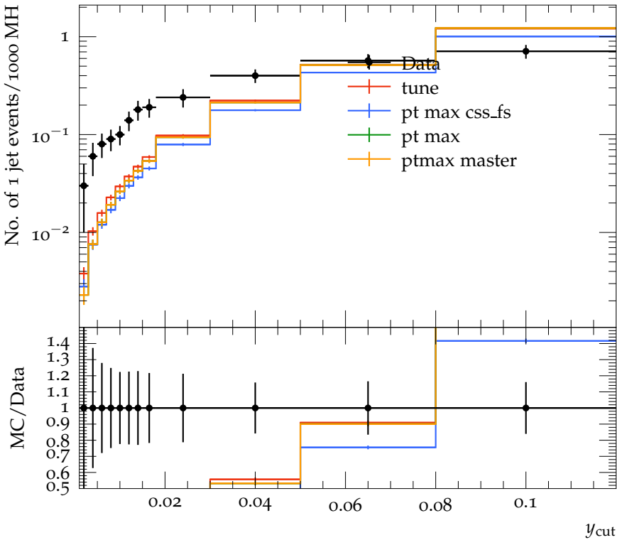
Number of 1 jet events vs y_{\text{cut}} , Durham
