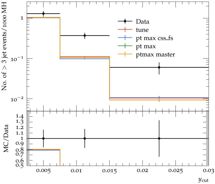
Number of > 3 jet events vs y_{\text{cut}} , Jade
