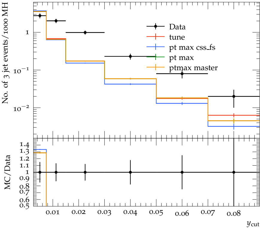
Number of 3 jet events vs y_{\text{cut}} , Jade
