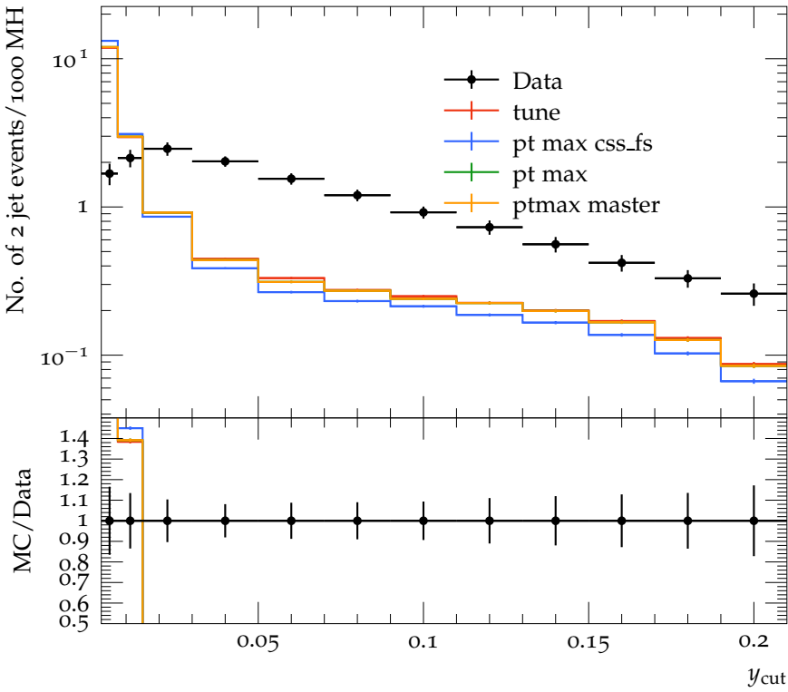
Number of 2 jet events vs y_{\text{cut}} , Jade
