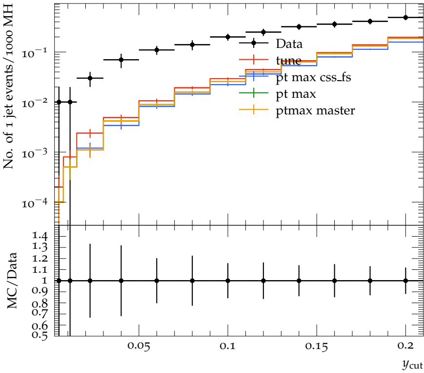
Number of 1 jet events vs y_{\text{cut}} , Jade
