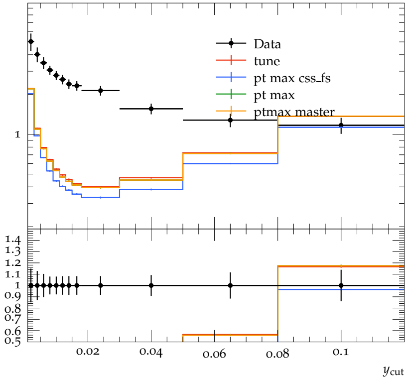
Number of photon vs y_{\text{cut}} , Durham
