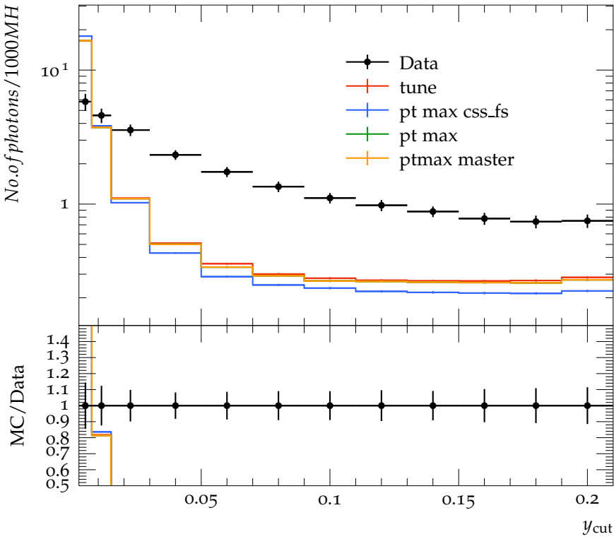
Number of photon vs y_{\text{cut}} , Jade
