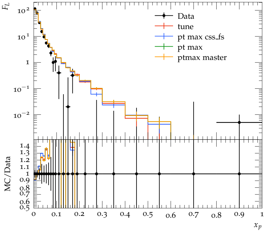
Longitudinal charged particle fragmentation function (uds)
