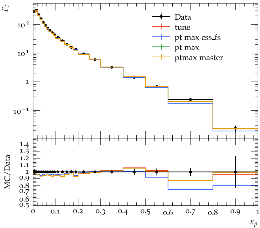
Transverse charged particle fragmentation function (uds)
