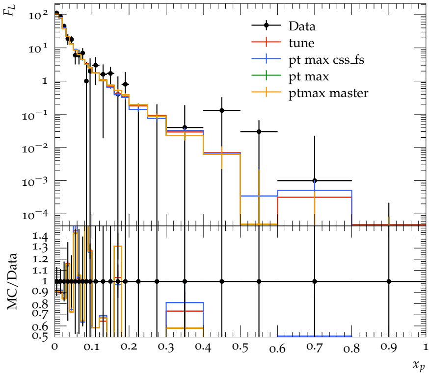
Longitudinal charged particle fragmentation function (bottom)
