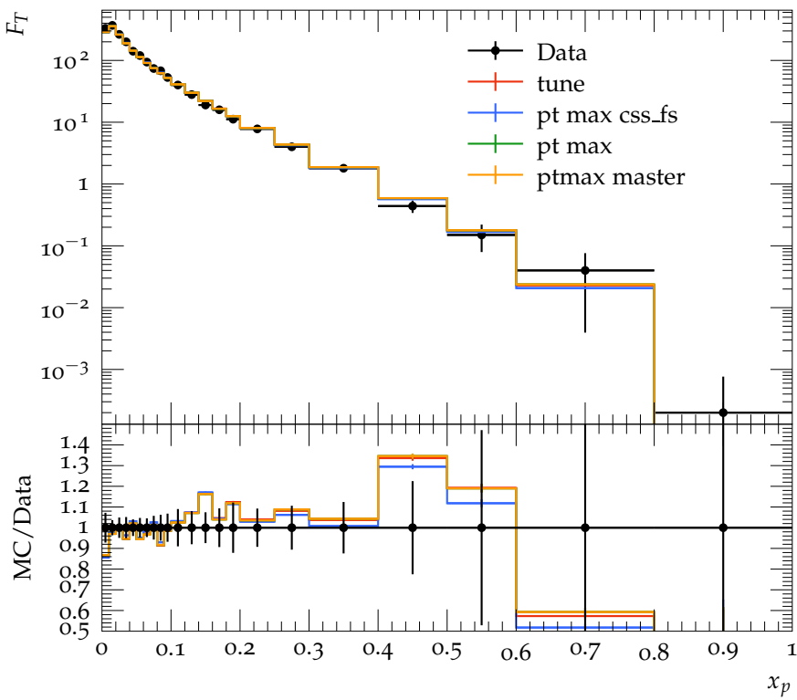
Transverse charged particle fragmentation function (bottom)
