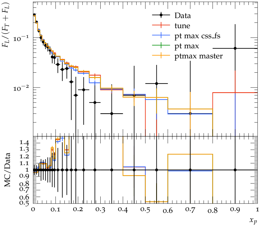
Ratio of Longitudinal and Longitudinal+Transverse fragmentation
