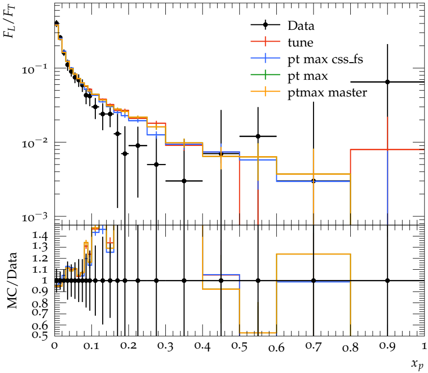
Ratio of Longitudinal and Transverse fragmentation function
