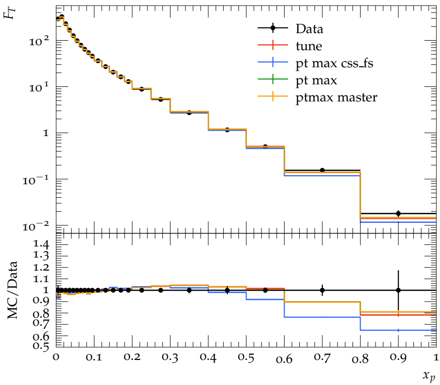
Transverse charged particle fragmentation function
