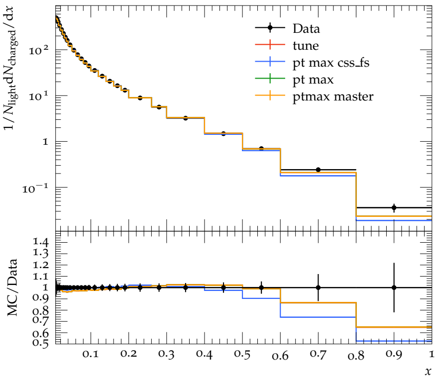
Charged Particle scaled momentum (light events)
