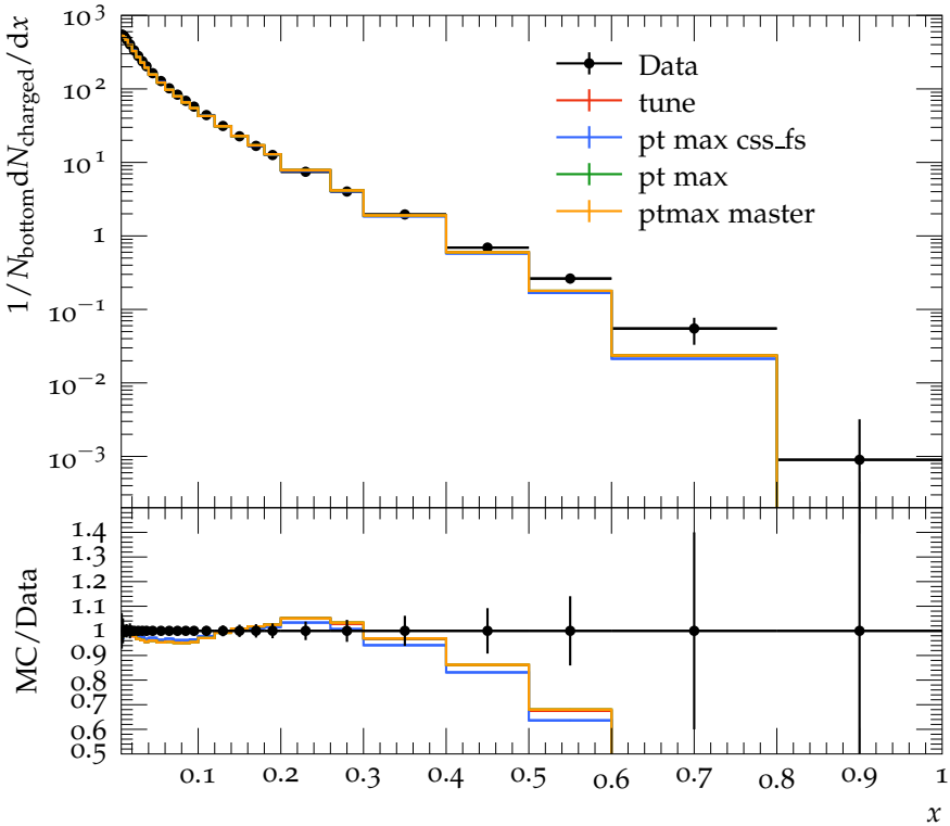
Charged Particle scaled momentum (bottom events)
