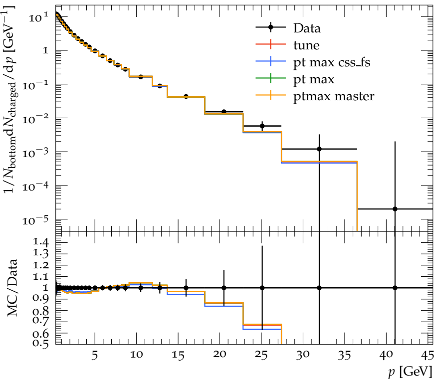
Charged Particle momentum (bottom events)
