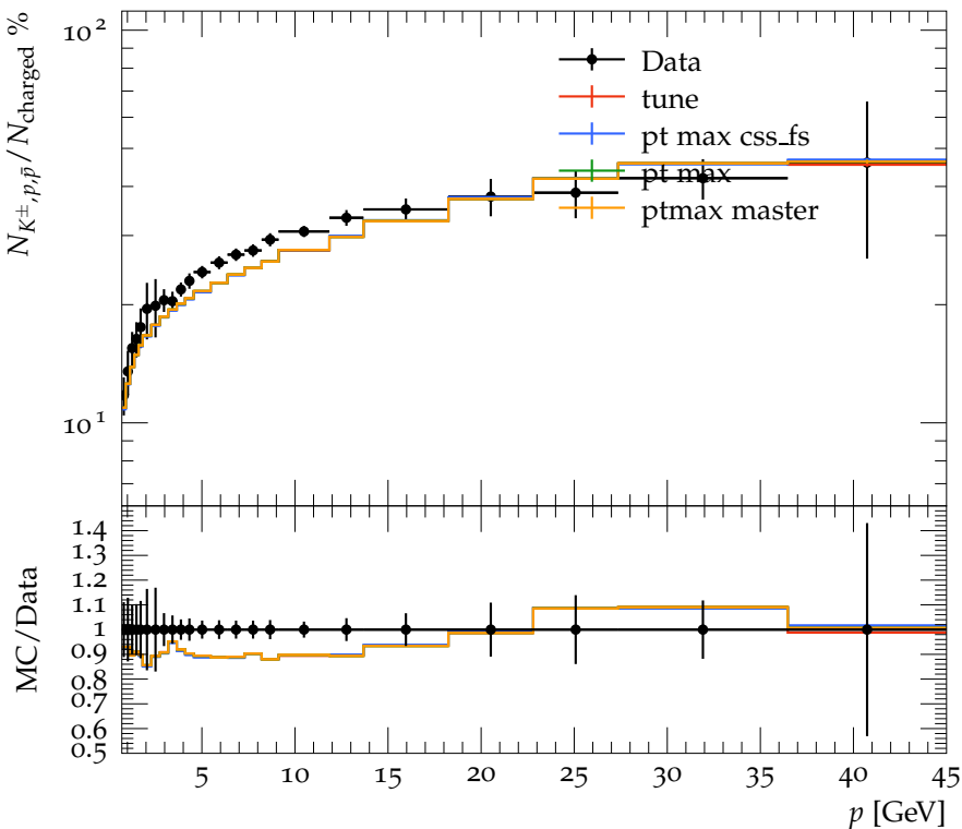
Ratio of N_{K^\pm, p, \bar{p}} to N_{\text{charged}} (light events)
