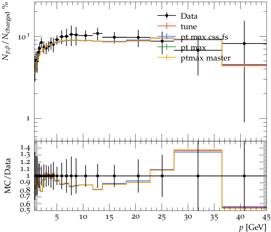
Ratio of N_{p,\bar{p}} to N_{\text{charged}} (light events)
