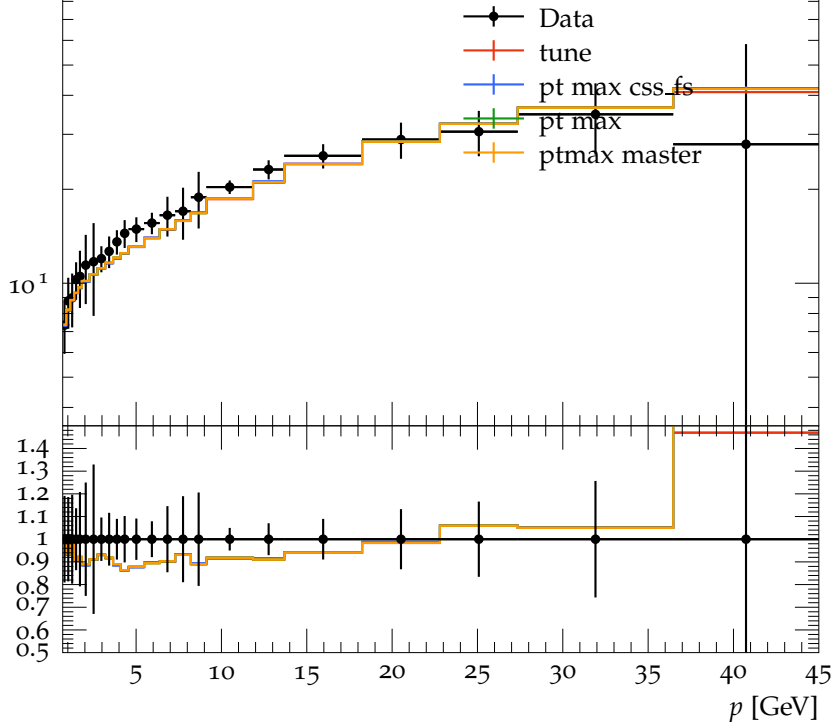
Ratio of N_{K^\pm} to N_{\text{charged}} (light events)
