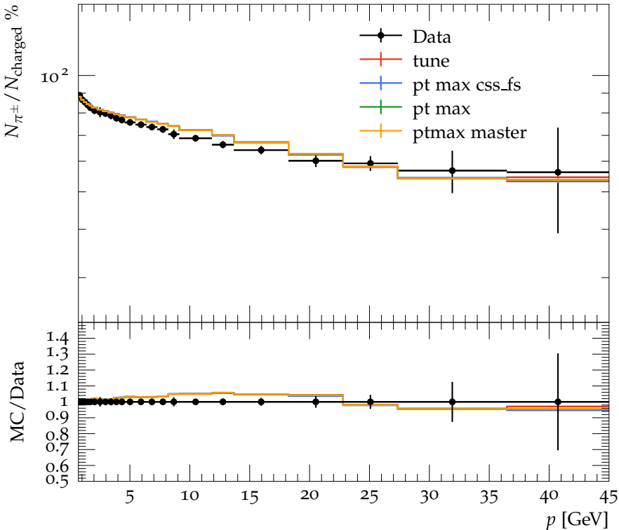
Ratio of N_{\pi^\pm} to N_{\text{charged}} (light events)
