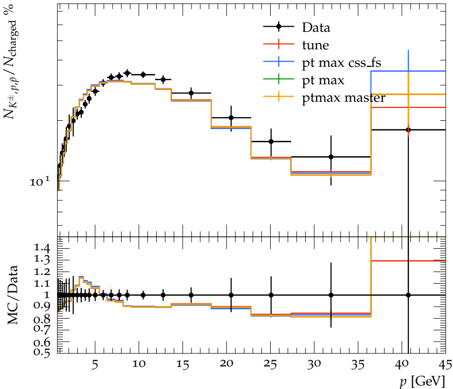
Ratio of N_{K^\pm, p, \bar{p}} to N_{\text{charged}} (bottom events)
