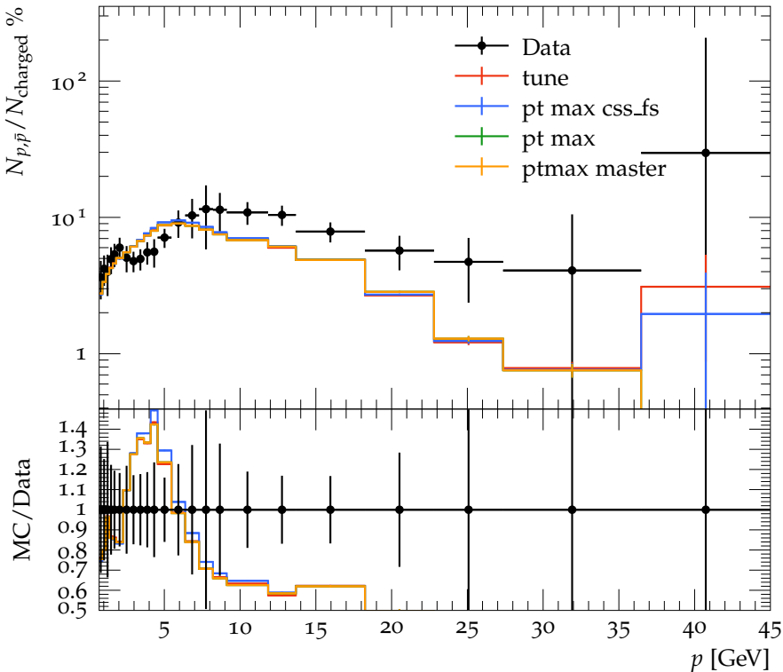
Ratio of N_{p,\bar{p}} to N_{\text{charged}} (bottom events)
