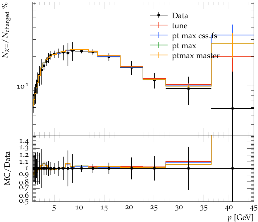
Ratio of N_{K^\pm} to N_{\text{charged}} (bottom events)
