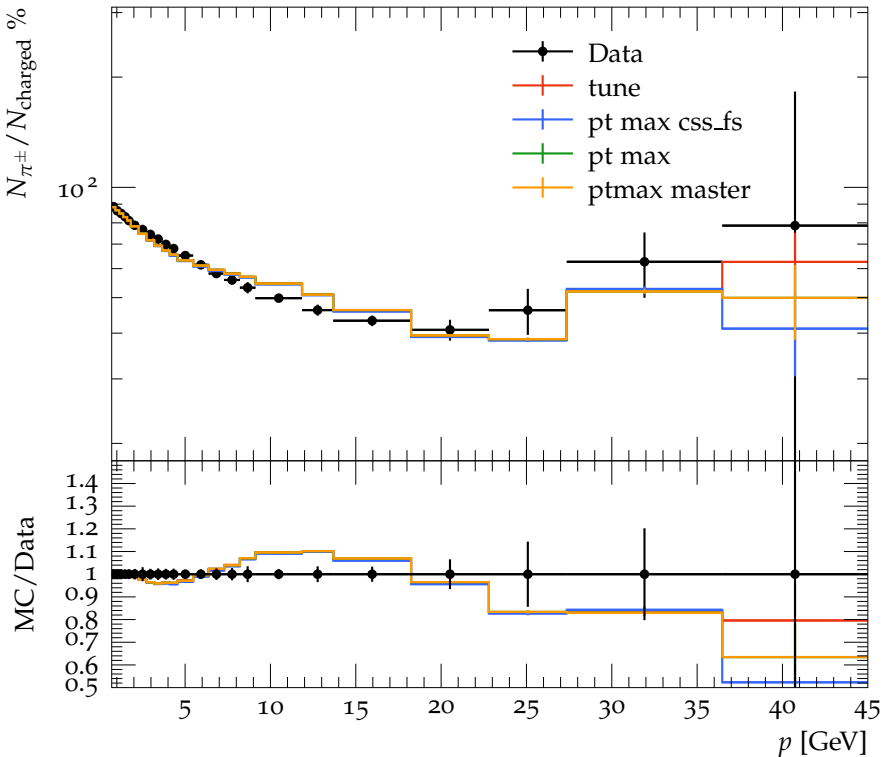
Ratio of N_{\pi^\pm} to N_{\text{charged}} (bottom events)
