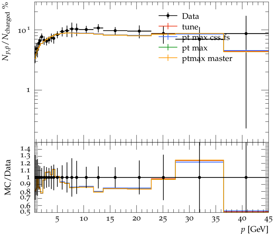
Ratio of N_{p,\bar{p}} to N_{\text{charged}} (all events)
