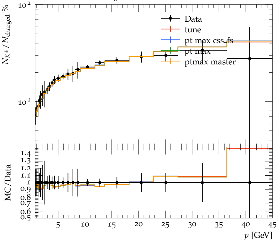
Ratio of N_{K^\pm} to N_{\text{charged}} (all events)
