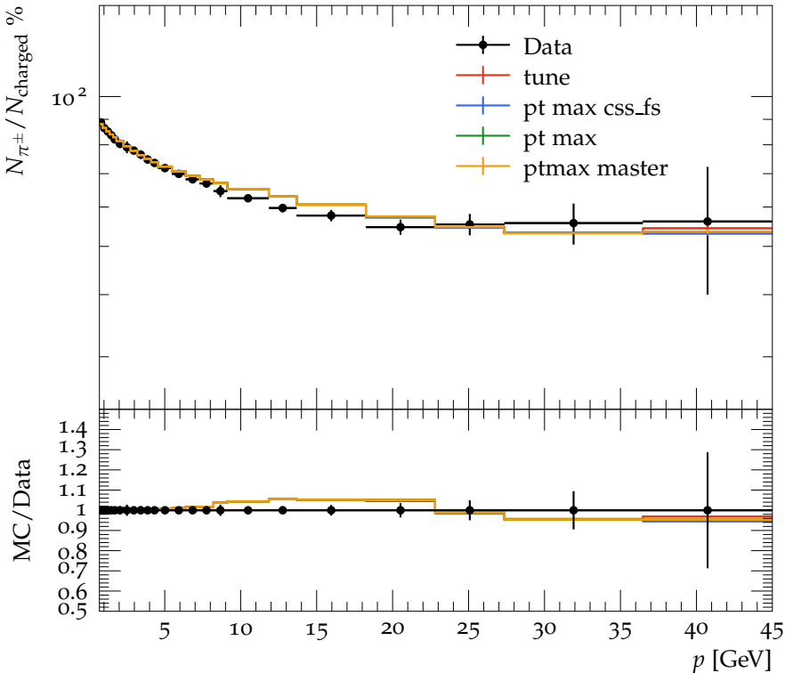
Ratio of N_{\pi^\pm} to N_{\text{charged}} (all events)
