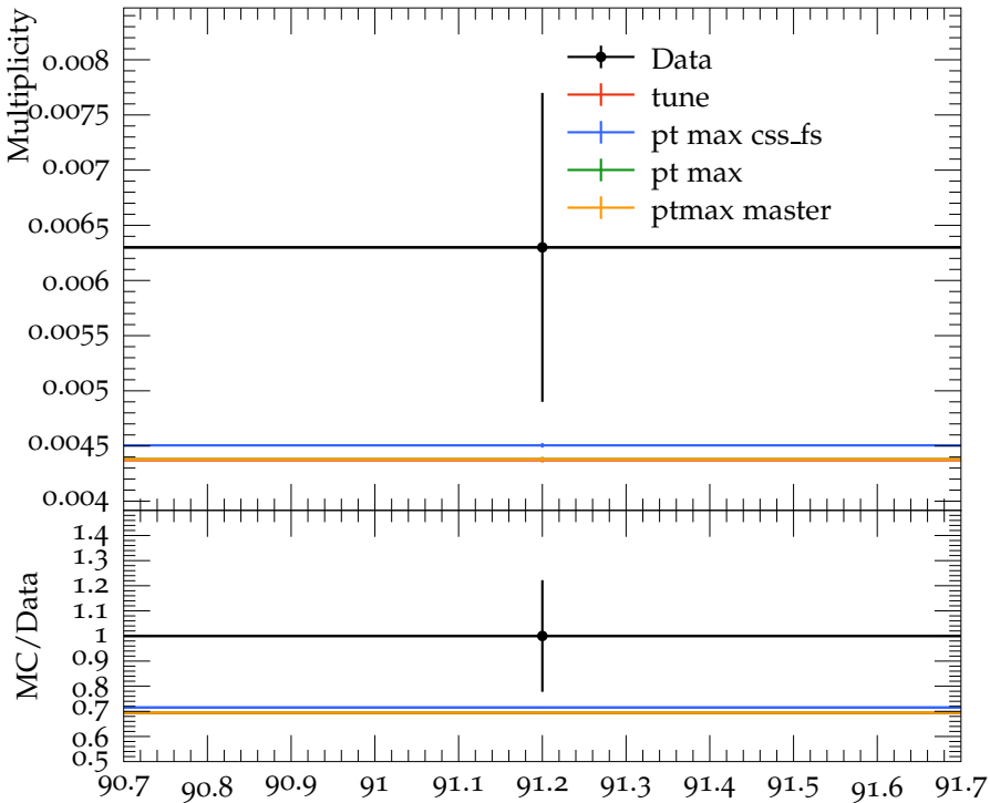
Mean \Xi(1530)^0 multiplicity
