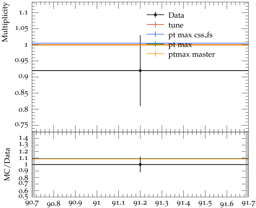
Mean p multiplicity
