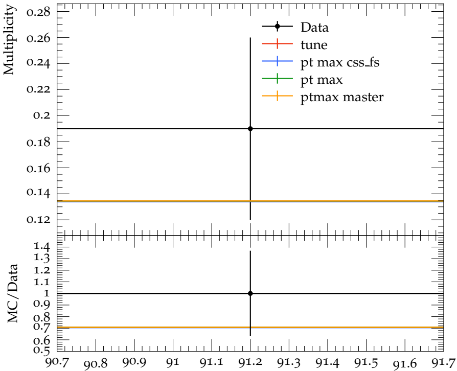
Mean K_2^*(1430)^0 multiplicity
