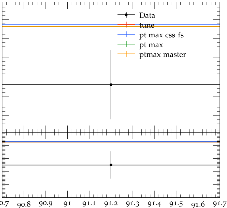
Mean \phi multiplicity
